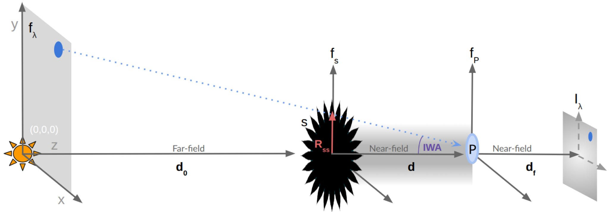
Figure 1. from Jamila S. Taaki et al 2026 Astron. J. 171 doi:10.3847/1538-3881/ae22f1 https://dx.doi.org/10.3847/1538-3881/ae22f1 © 2025. The Author(s). Published by the American Astronomical Society.
