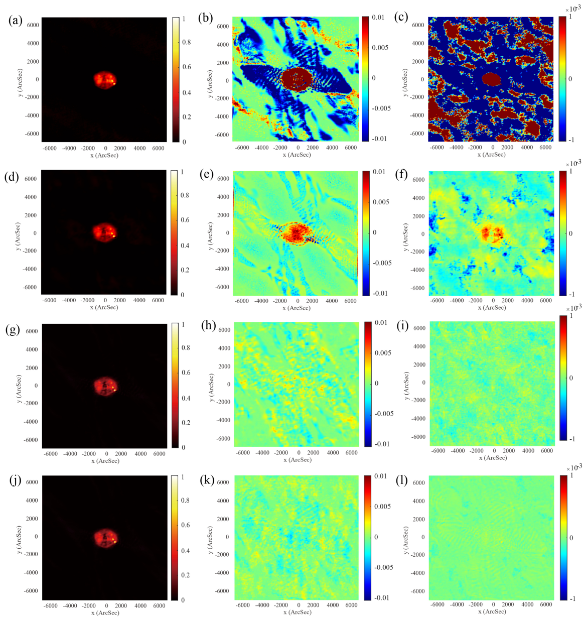
Figure 9. from Xiaocheng Yang et al 2026 Astron. J. 171 doi:10.3847/1538-3881/ae22d7 https://dx.doi.org/10.3847/1538-3881/ae22d7 © 2025. The Author(s). Published by the American Astronomical Society.
