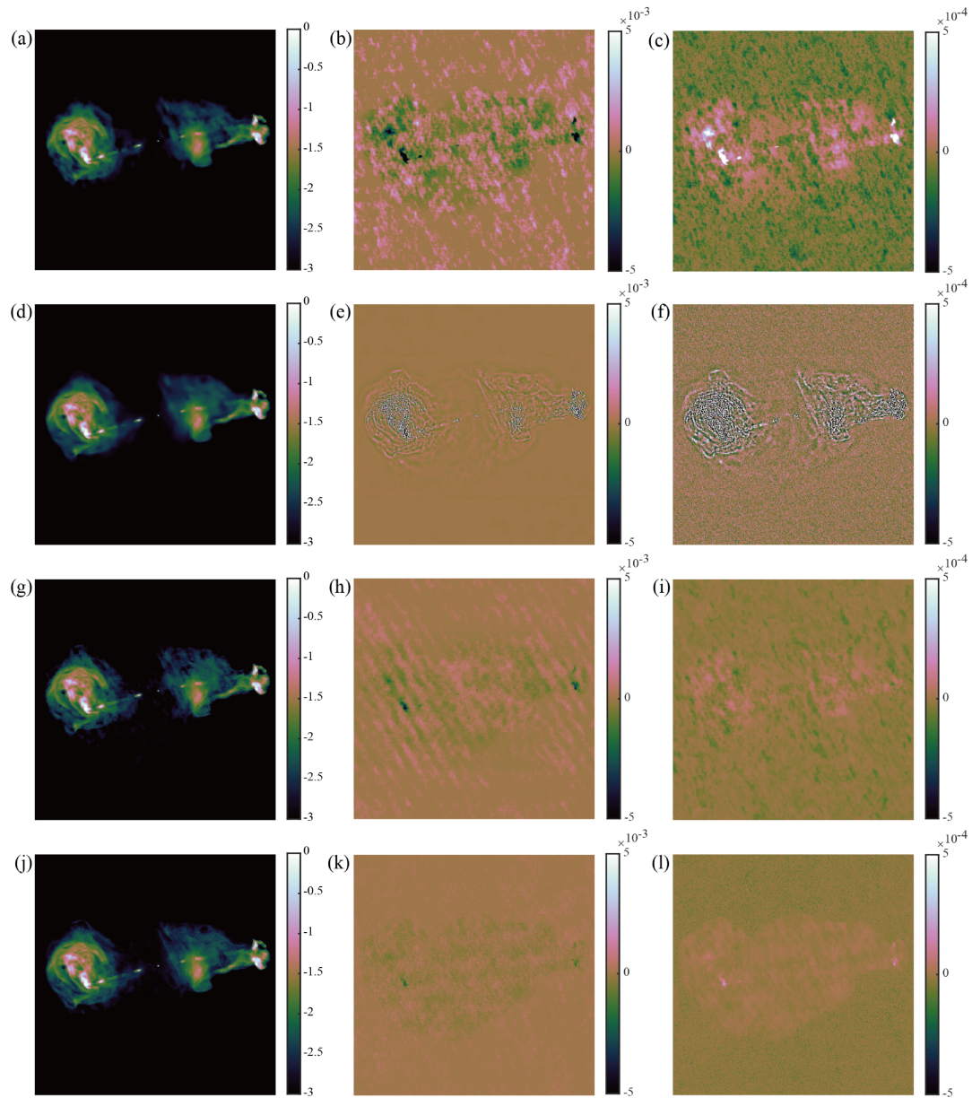
Figure 7. from Xiaocheng Yang et al 2026 Astron. J. 171 doi:10.3847/1538-3881/ae22d7 https://dx.doi.org/10.3847/1538-3881/ae22d7 © 2025. The Author(s). Published by the American Astronomical Society.
