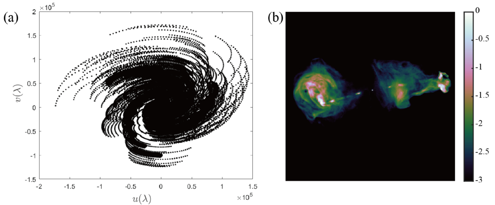
Figure 6. from Xiaocheng Yang et al 2026 Astron. J. 171 doi:10.3847/1538-3881/ae22d7 https://dx.doi.org/10.3847/1538-3881/ae22d7 © 2025. The Author(s). Published by the American Astronomical Society.
