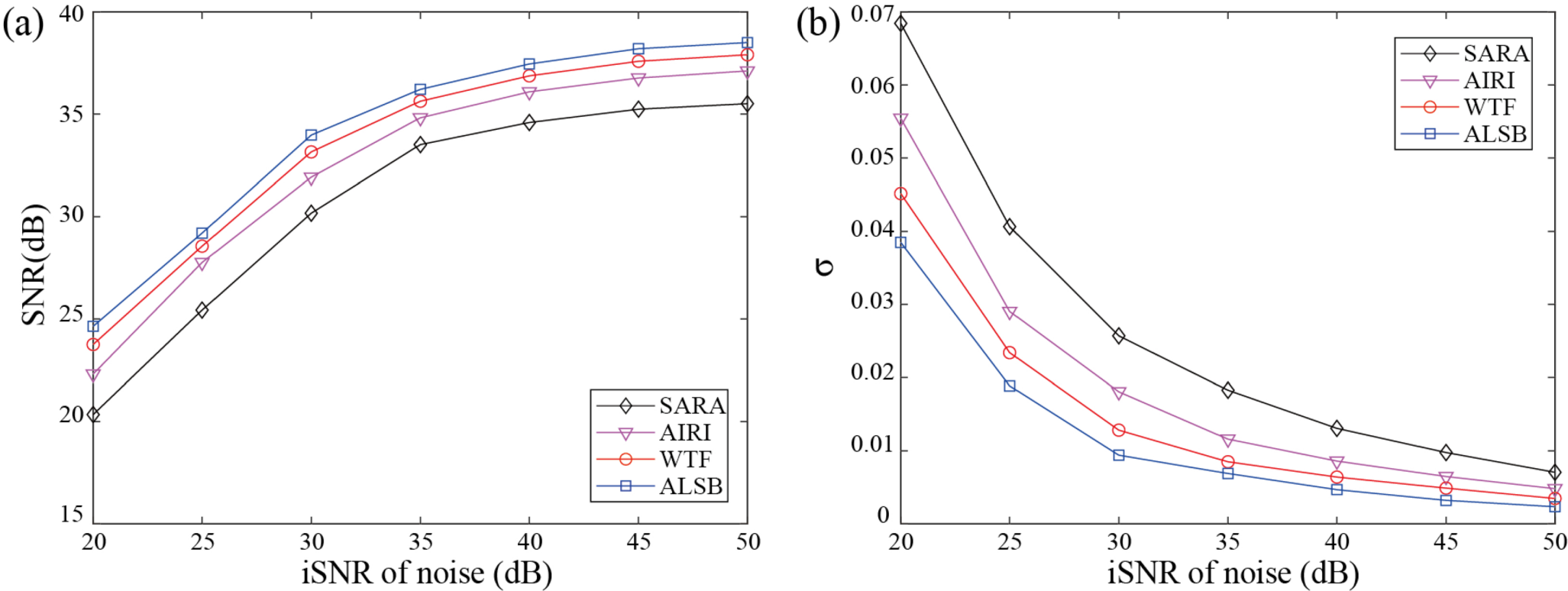
Figure 5. from Xiaocheng Yang et al 2026 Astron. J. 171 doi:10.3847/1538-3881/ae22d7 https://dx.doi.org/10.3847/1538-3881/ae22d7 © 2025. The Author(s). Published by the American Astronomical Society.
