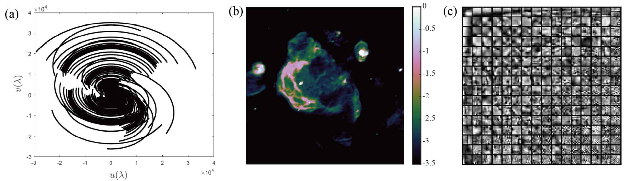
Figure 1. from Xiaocheng Yang et al 2026 Astron. J. 171 doi:10.3847/1538-3881/ae22d7 https://dx.doi.org/10.3847/1538-3881/ae22d7 © 2025. The Author(s). Published by the American Astronomical Society.
