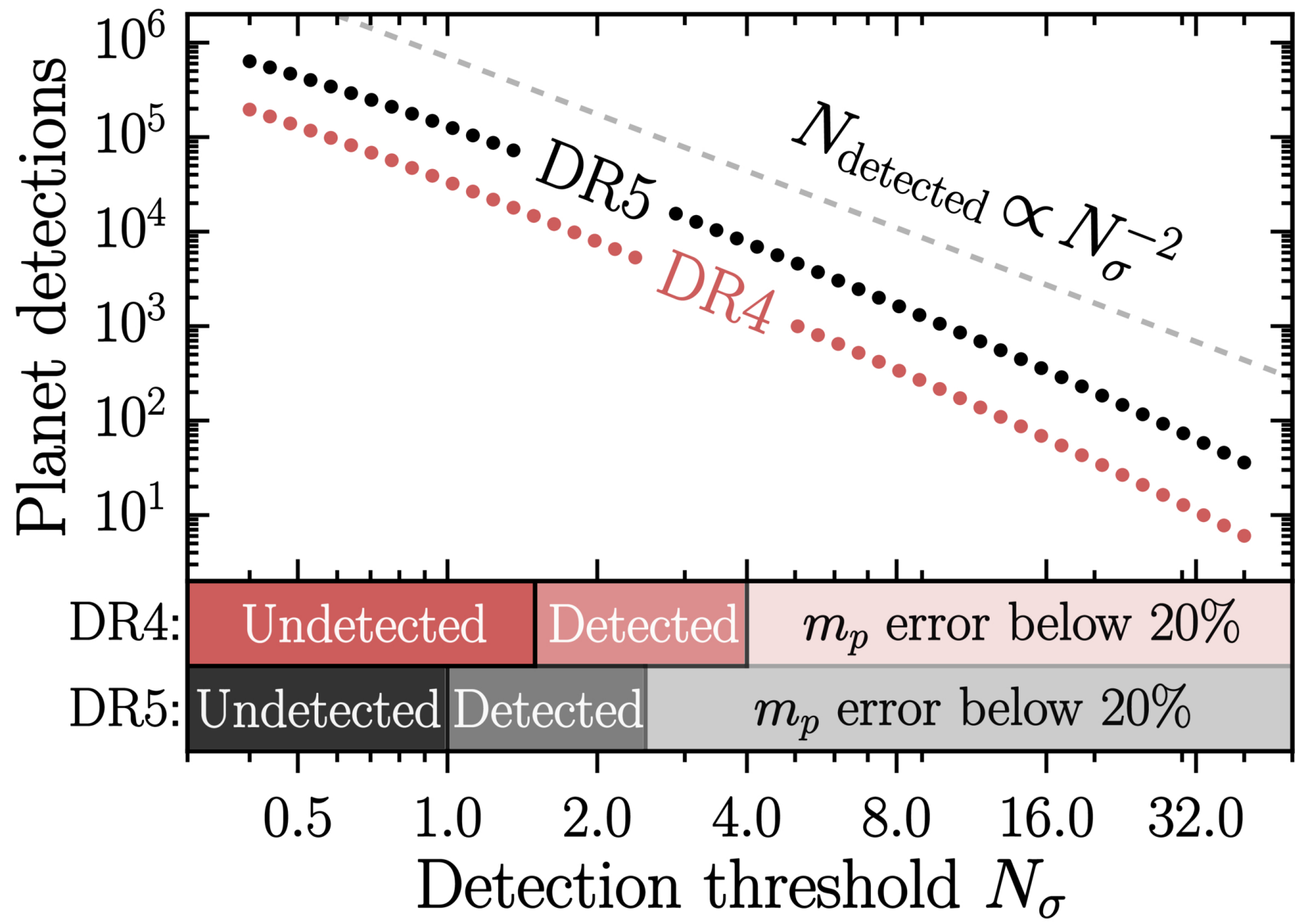
Figure 8. from Caleb Lammers and Joshua N. Winn 2026 Astron. J. 171 doi:10.3847/1538-3881/ae21de https://dx.doi.org/10.3847/1538-3881/ae21de © 2025. The Author(s). Published by the American Astronomical Society.
