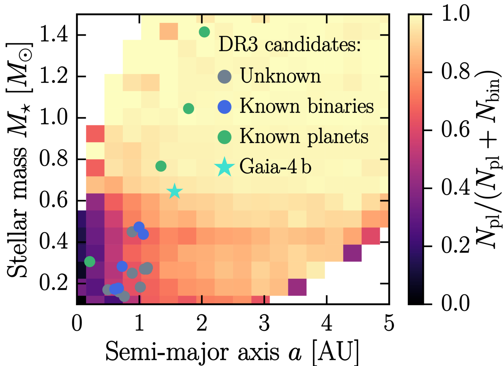
Figure 14. from Caleb Lammers and Joshua N. Winn 2026 Astron. J. 171 doi:10.3847/1538-3881/ae21de https://dx.doi.org/10.3847/1538-3881/ae21de © 2025. The Author(s). Published by the American Astronomical Society.
