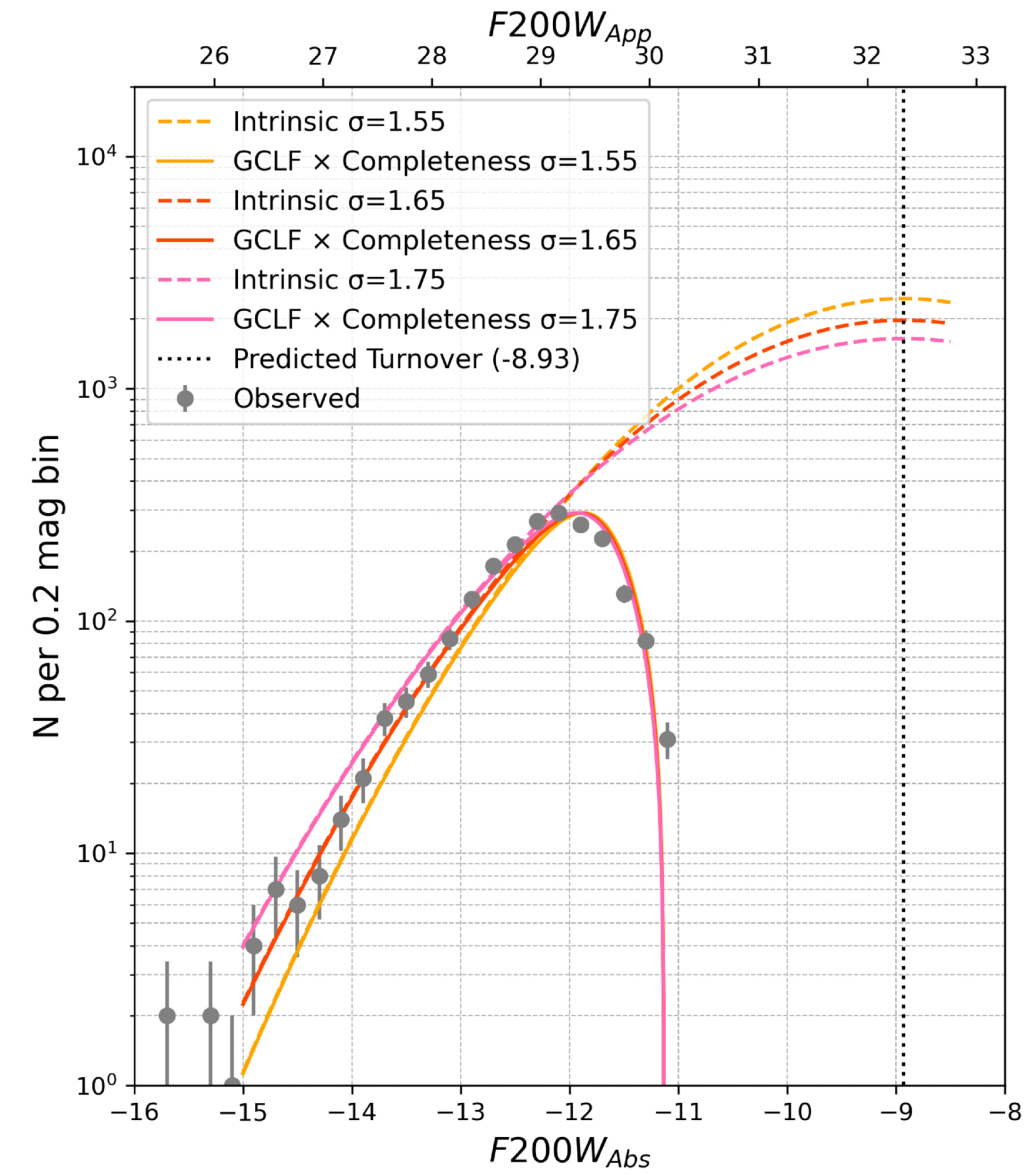
Figure 7. from Jessica M. Berkheimer et al 2026 Astron. J. 171 doi:10.3847/1538-3881/ae209a https://dx.doi.org/10.3847/1538-3881/ae209a © 2025. The Author(s). Published by the American Astronomical Society.
