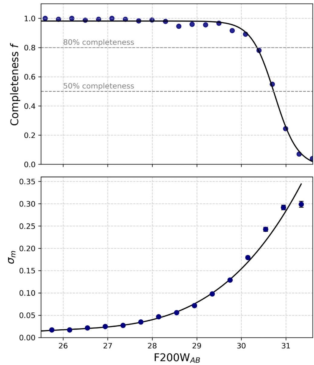
Figure 3. from Jessica M. Berkheimer et al 2026 Astron. J. 171 doi:10.3847/1538-3881/ae209a https://dx.doi.org/10.3847/1538-3881/ae209a © 2025. The Author(s). Published by the American Astronomical Society.
