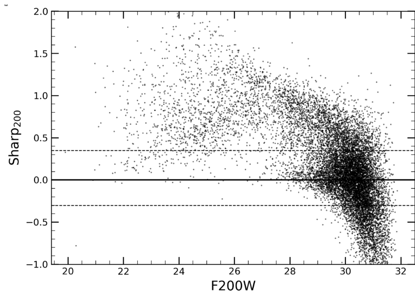
Figure 2. from Jessica M. Berkheimer et al 2026 Astron. J. 171 doi:10.3847/1538-3881/ae209a https://dx.doi.org/10.3847/1538-3881/ae209a © 2025. The Author(s). Published by the American Astronomical Society.
