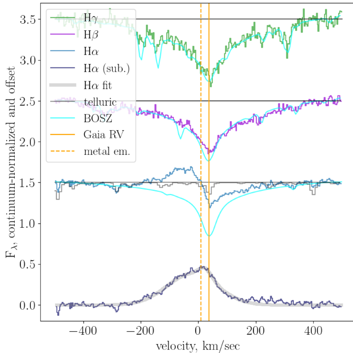
Figure 9. from Nadia L. Zakamska et al 2026 Astron. J. 171 doi:10.3847/1538-3881/ae1fd9 https://dx.doi.org/10.3847/1538-3881/ae1fd9 © 2026. The Author(s). Published by the American Astronomical Society.
