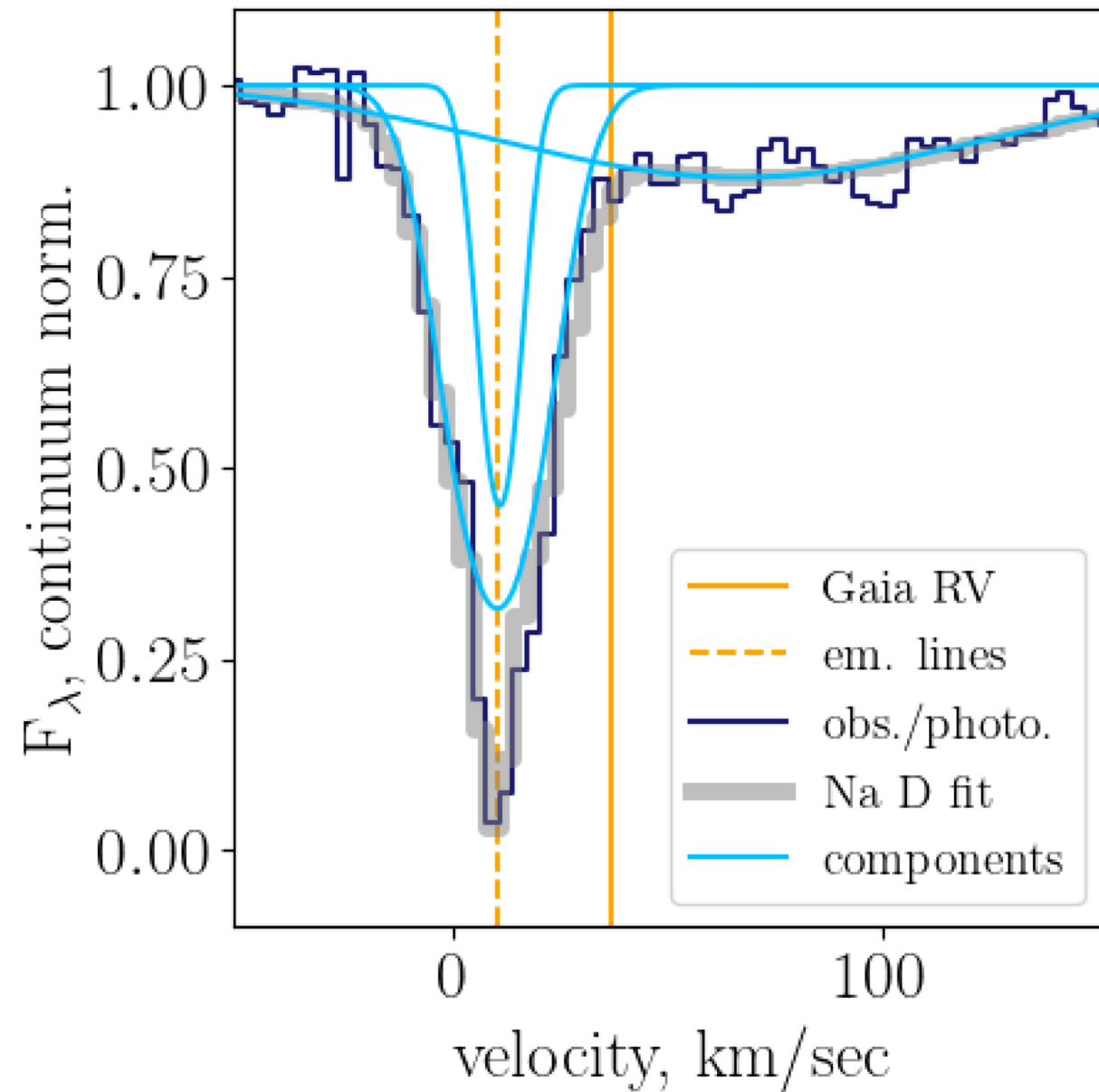
Figure 8. from Nadia L. Zakamska et al 2026 Astron. J. 171 doi:10.3847/1538-3881/ae1fd9 https://dx.doi.org/10.3847/1538-3881/ae1fd9 © 2026. The Author(s). Published by the American Astronomical Society.
