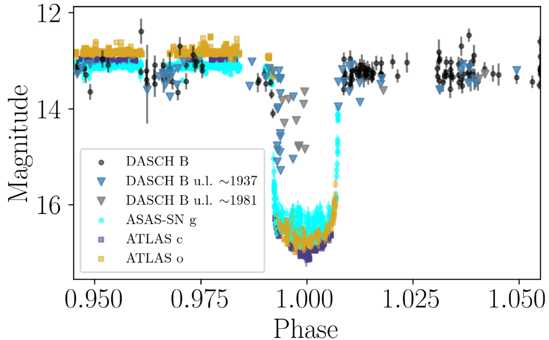
Figure 6. from Nadia L. Zakamska et al 2026 Astron. J. 171 doi:10.3847/1538-3881/ae1fd9 https://dx.doi.org/10.3847/1538-3881/ae1fd9 © 2026. The Author(s). Published by the American Astronomical Society.
