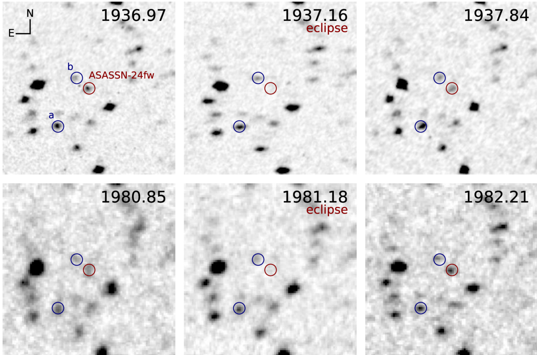
Figure 5. from Nadia L. Zakamska et al 2026 Astron. J. 171 doi:10.3847/1538-3881/ae1fd9 https://dx.doi.org/10.3847/1538-3881/ae1fd9 © 2026. The Author(s). Published by the American Astronomical Society.
