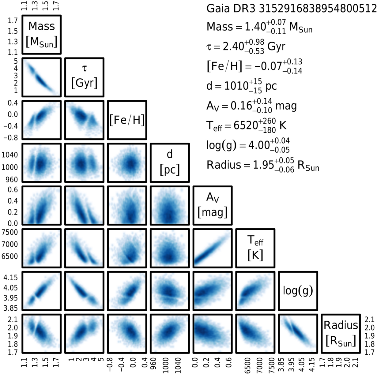
Figure 2. from Nadia L. Zakamska et al 2026 Astron. J. 171 doi:10.3847/1538-3881/ae1fd9 https://dx.doi.org/10.3847/1538-3881/ae1fd9 © 2026. The Author(s). Published by the American Astronomical Society.
