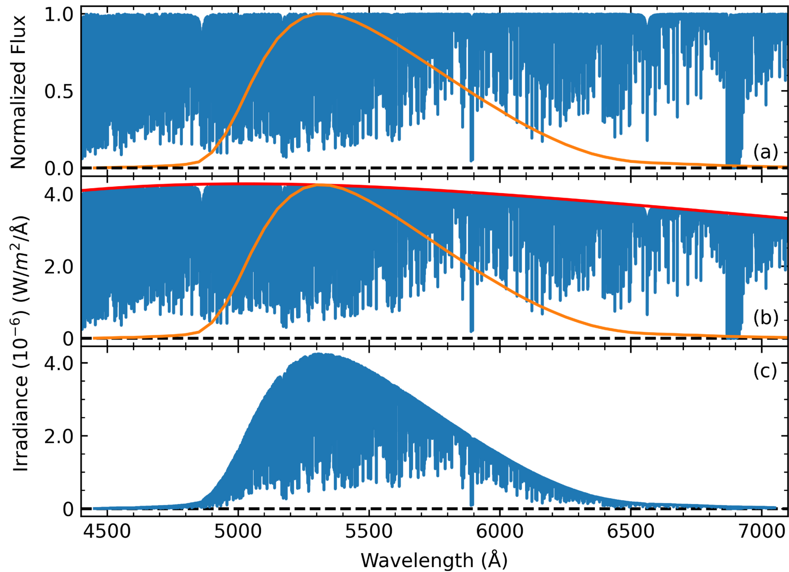
Figure 2. from Gökhan Yücel et al 2026 Astron. J. 171 doi:10.3847/1538-3881/ae1f8c https://dx.doi.org/10.3847/1538-3881/ae1f8c © 2025. The Author(s). Published by the American Astronomical Society.
