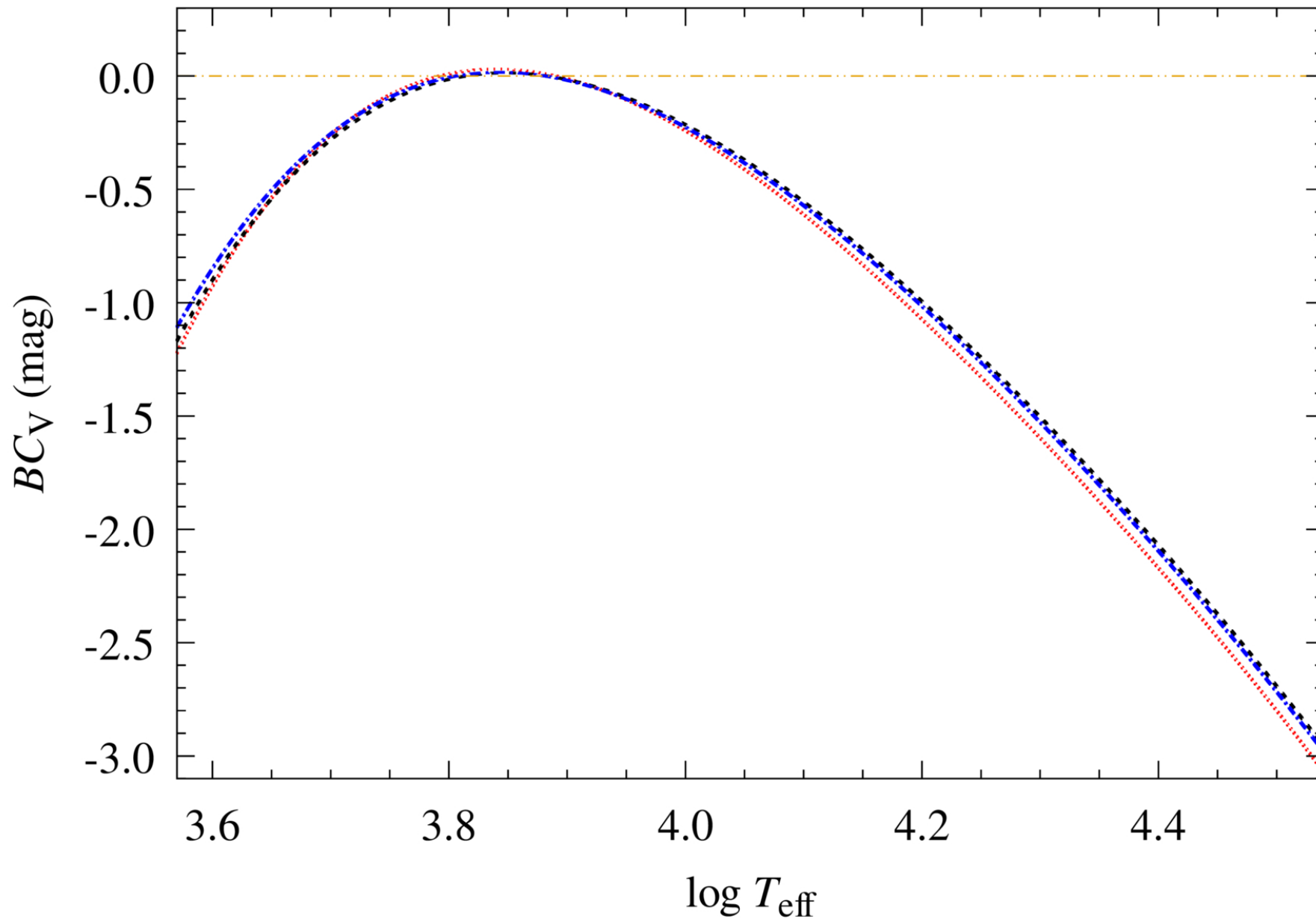
Figure 10. from Gökhan Yücel et al 2026 Astron. J. 171 doi:10.3847/1538-3881/ae1f8c https://dx.doi.org/10.3847/1538-3881/ae1f8c © 2025. The Author(s). Published by the American Astronomical Society.
