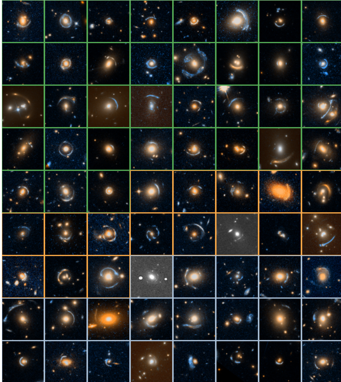
Figure 3. from Tania M. Barone et al 2026 Astron. J. 171 doi:10.3847/1538-3881/ae1f86 https://dx.doi.org/10.3847/1538-3881/ae1f86 © 2025. The Author(s). Published by the American Astronomical Society.
