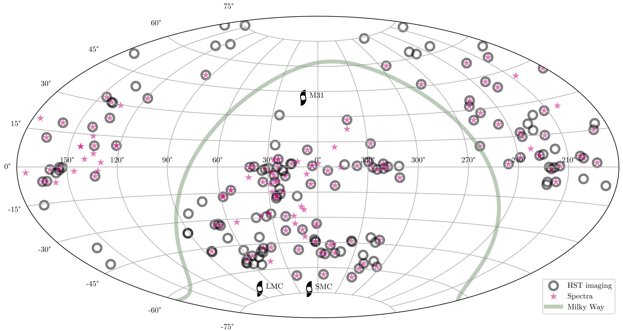
Figure 2. from Tania M. Barone et al 2026 Astron. J. 171 doi:10.3847/1538-3881/ae1f86 https://dx.doi.org/10.3847/1538-3881/ae1f86 © 2025. The Author(s). Published by the American Astronomical Society.
