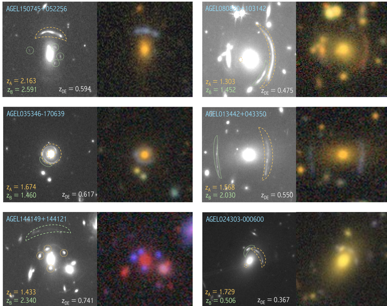
Figure 13. from Tania M. Barone et al 2026 Astron. J. 171 doi:10.3847/1538-3881/ae1f86 https://dx.doi.org/10.3847/1538-3881/ae1f86 © 2025. The Author(s). Published by the American Astronomical Society.
