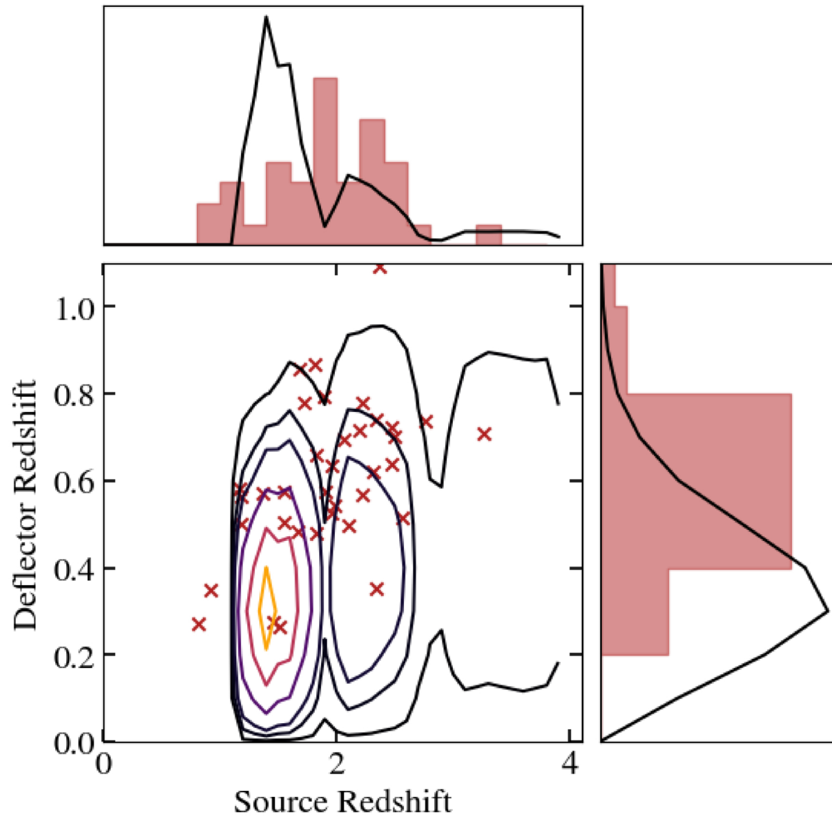
Figure 12. from Tania M. Barone et al 2026 Astron. J. 171 doi:10.3847/1538-3881/ae1f86 https://dx.doi.org/10.3847/1538-3881/ae1f86 © 2025. The Author(s). Published by the American Astronomical Society.
