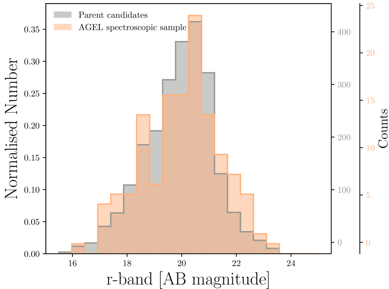
Figure 10. from Tania M. Barone et al 2026 Astron. J. 171 doi:10.3847/1538-3881/ae1f86 https://dx.doi.org/10.3847/1538-3881/ae1f86 © 2025. The Author(s). Published by the American Astronomical Society.
