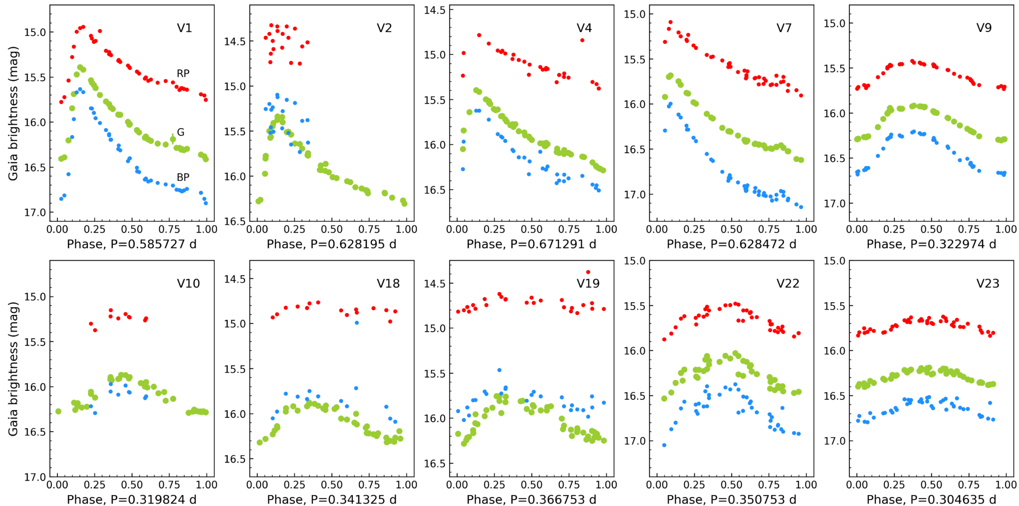
Figure 3. from Csilla Kalup and László Molnár 2026 Astron. J. 171 doi:10.3847/1538-3881/ae1f0f https://dx.doi.org/10.3847/1538-3881/ae1f0f © 2025. The Author(s). Published by the American Astronomical Society.
