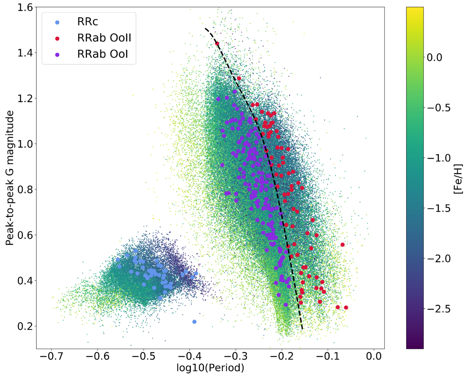
Figure 2. from Csilla Kalup and László Molnár 2026 Astron. J. 171 doi:10.3847/1538-3881/ae1f0f https://dx.doi.org/10.3847/1538-3881/ae1f0f © 2025. The Author(s). Published by the American Astronomical Society.
