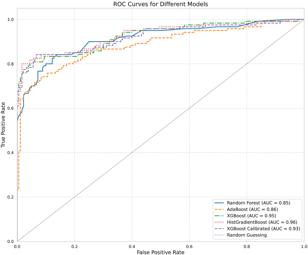
Figure 4. from Mir Sakhawat Hossain and Md. Sadman 2026 Astron. J. 171 doi:10.3847/1538-3881/ae1ba3 https://dx.doi.org/10.3847/1538-3881/ae1ba3 © 2025. The Author(s). Published by the American Astronomical Society.
