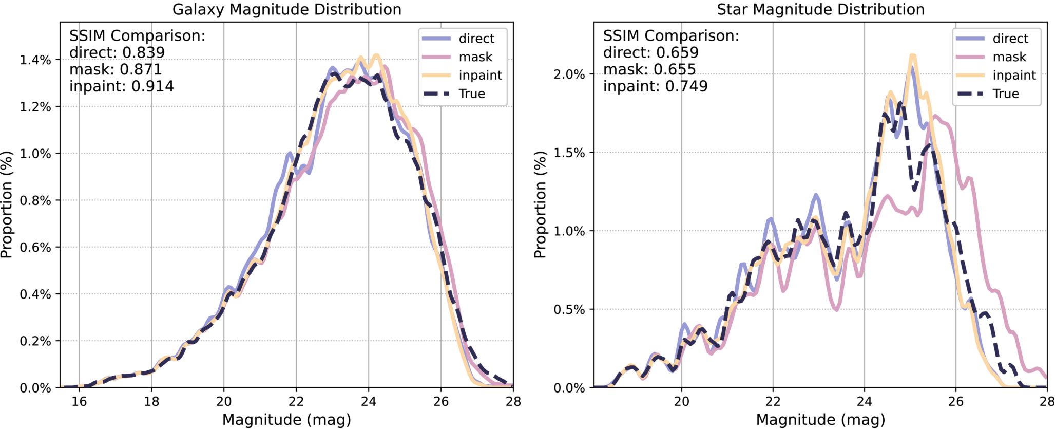
Figure 7. from Yan Yu et al 2026 Astron. J. 171 doi:10.3847/1538-3881/ae1b96 https://dx.doi.org/10.3847/1538-3881/ae1b96 © 2025. The Author(s). Published by the American Astronomical Society.
