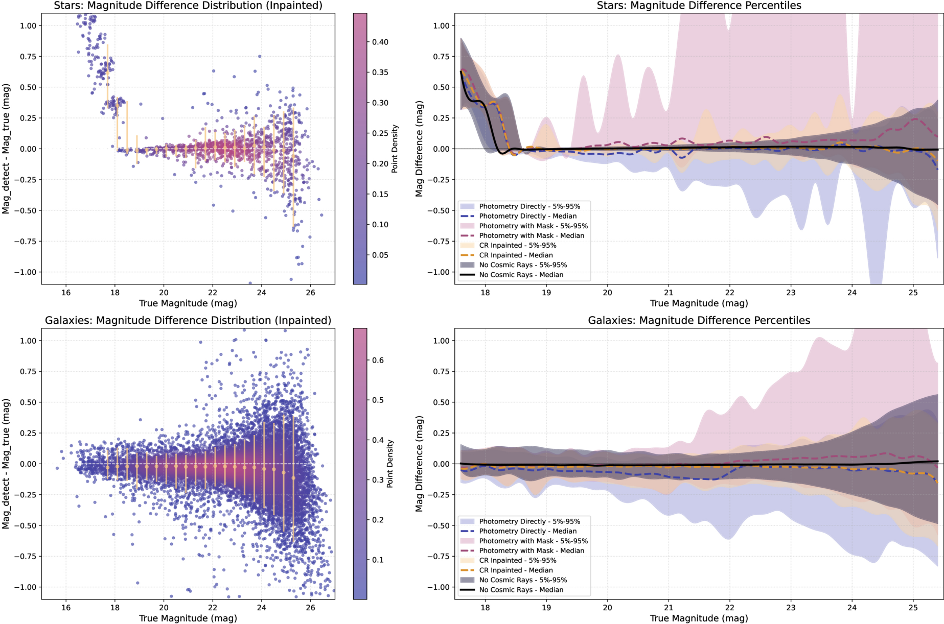
Figure 6. from Yan Yu et al 2026 Astron. J. 171 doi:10.3847/1538-3881/ae1b96 https://dx.doi.org/10.3847/1538-3881/ae1b96 © 2025. The Author(s). Published by the American Astronomical Society.
