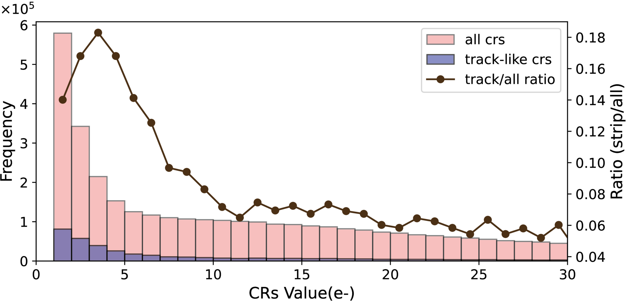
Figure 4. from Yan Yu et al 2026 Astron. J. 171 doi:10.3847/1538-3881/ae1b96 https://dx.doi.org/10.3847/1538-3881/ae1b96 © 2025. The Author(s). Published by the American Astronomical Society.
