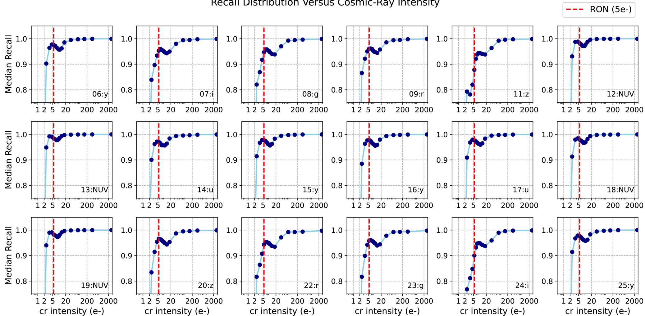
Figure 3. from Yan Yu et al 2026 Astron. J. 171 doi:10.3847/1538-3881/ae1b96 https://dx.doi.org/10.3847/1538-3881/ae1b96 © 2025. The Author(s). Published by the American Astronomical Society.
