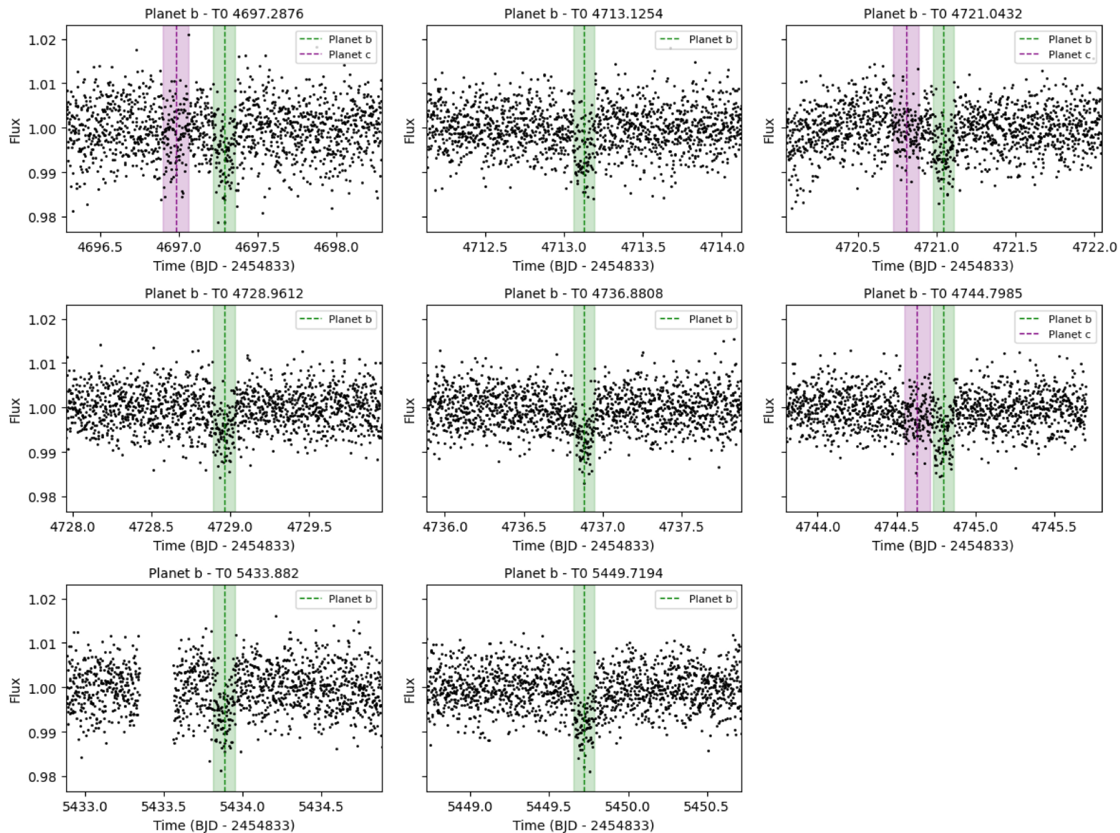
Figure 8. from Paige M. Entrican et al 2026 Astron. J. 171 doi:10.3847/1538-3881/ae1b90 https://dx.doi.org/10.3847/1538-3881/ae1b90 © 2025. The Author(s). Published by the American Astronomical Society.
