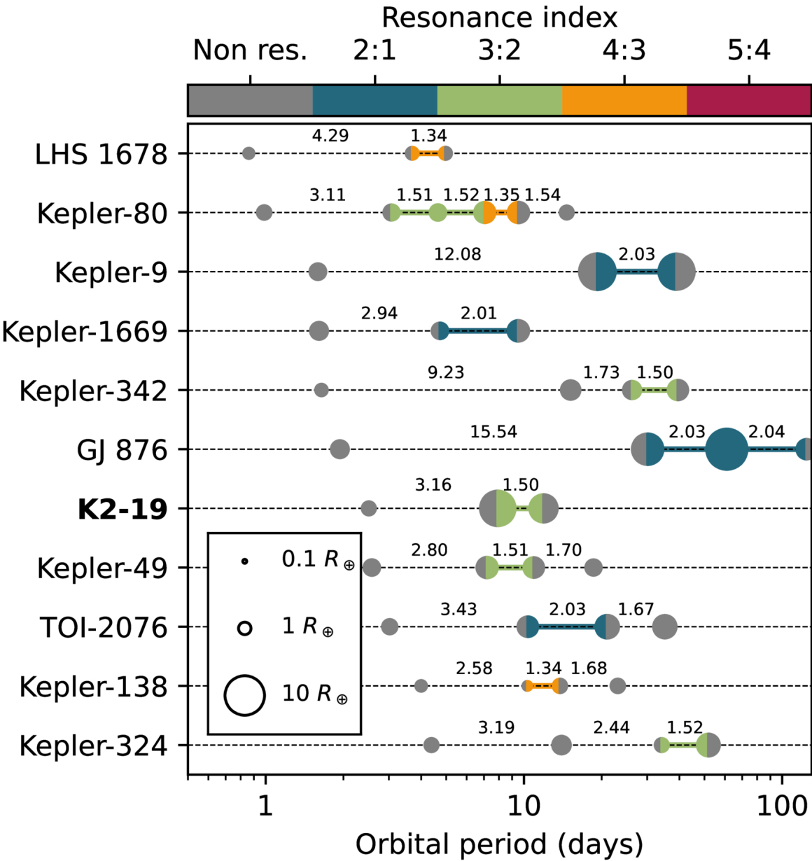
Figure 7. from Paige M. Entrican et al 2026 Astron. J. 171 doi:10.3847/1538-3881/ae1b90 https://dx.doi.org/10.3847/1538-3881/ae1b90 © 2025. The Author(s). Published by the American Astronomical Society.
