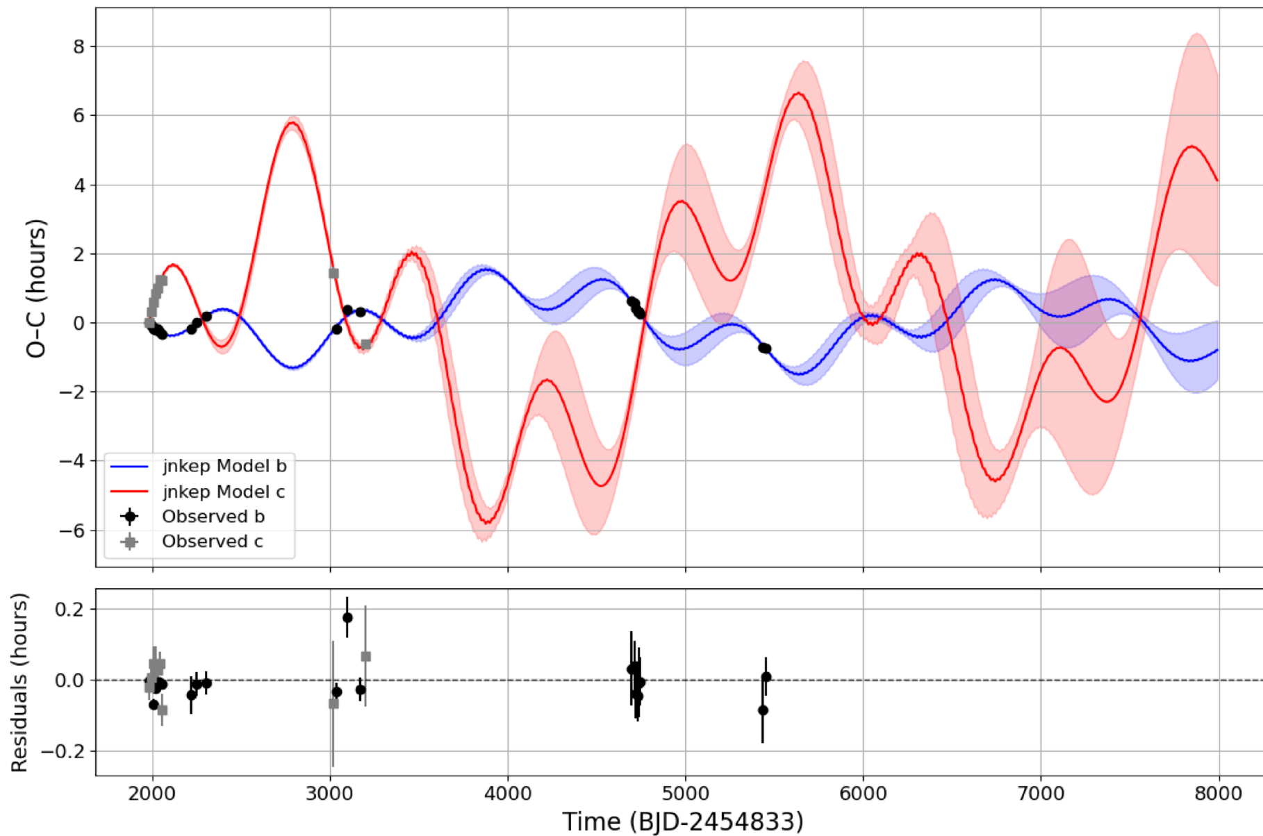
Figure 3. from Paige M. Entrican et al 2026 Astron. J. 171 doi:10.3847/1538-3881/ae1b90 https://dx.doi.org/10.3847/1538-3881/ae1b90 © 2025. The Author(s). Published by the American Astronomical Society.
