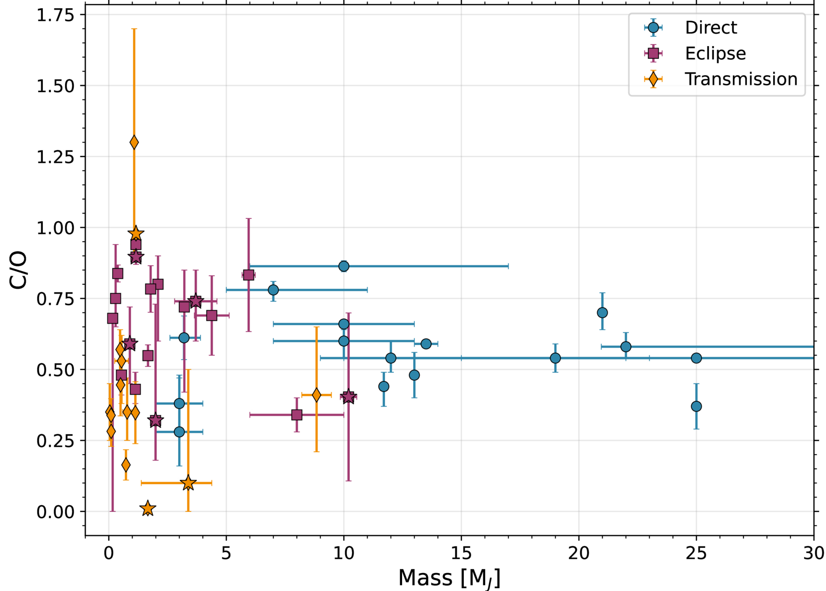
Figure 9. from Joshua D. Lothringer et al 2026 Astron. J. 171 doi:10.3847/1538-3881/ae1b8e https://dx.doi.org/10.3847/1538-3881/ae1b8e © 2025. The Author(s). Published by the American Astronomical Society.
