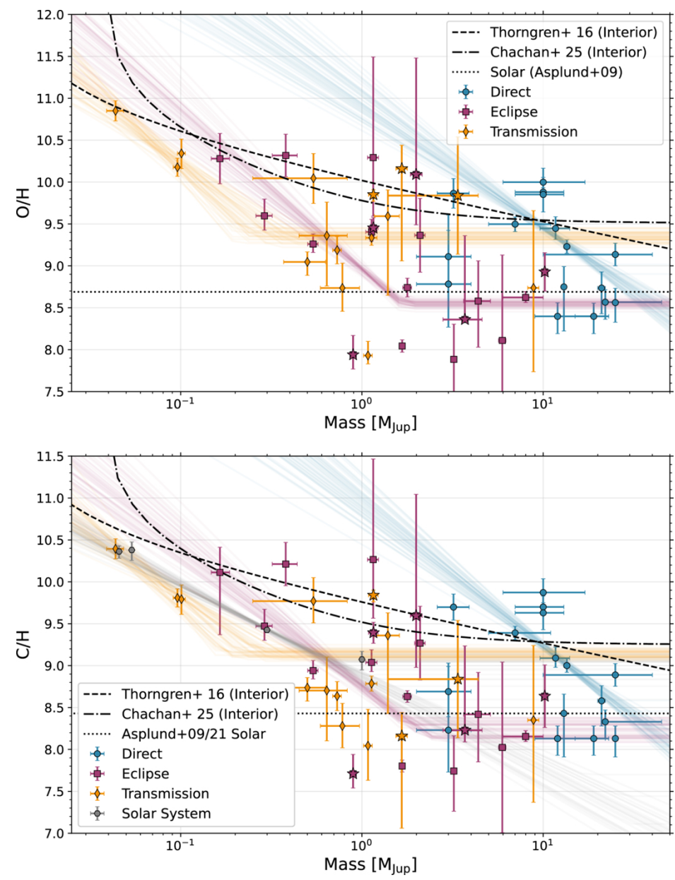
Figure 6. from Joshua D. Lothringer et al 2026 Astron. J. 171 doi:10.3847/1538-3881/ae1b8e https://dx.doi.org/10.3847/1538-3881/ae1b8e © 2025. The Author(s). Published by the American Astronomical Society.
