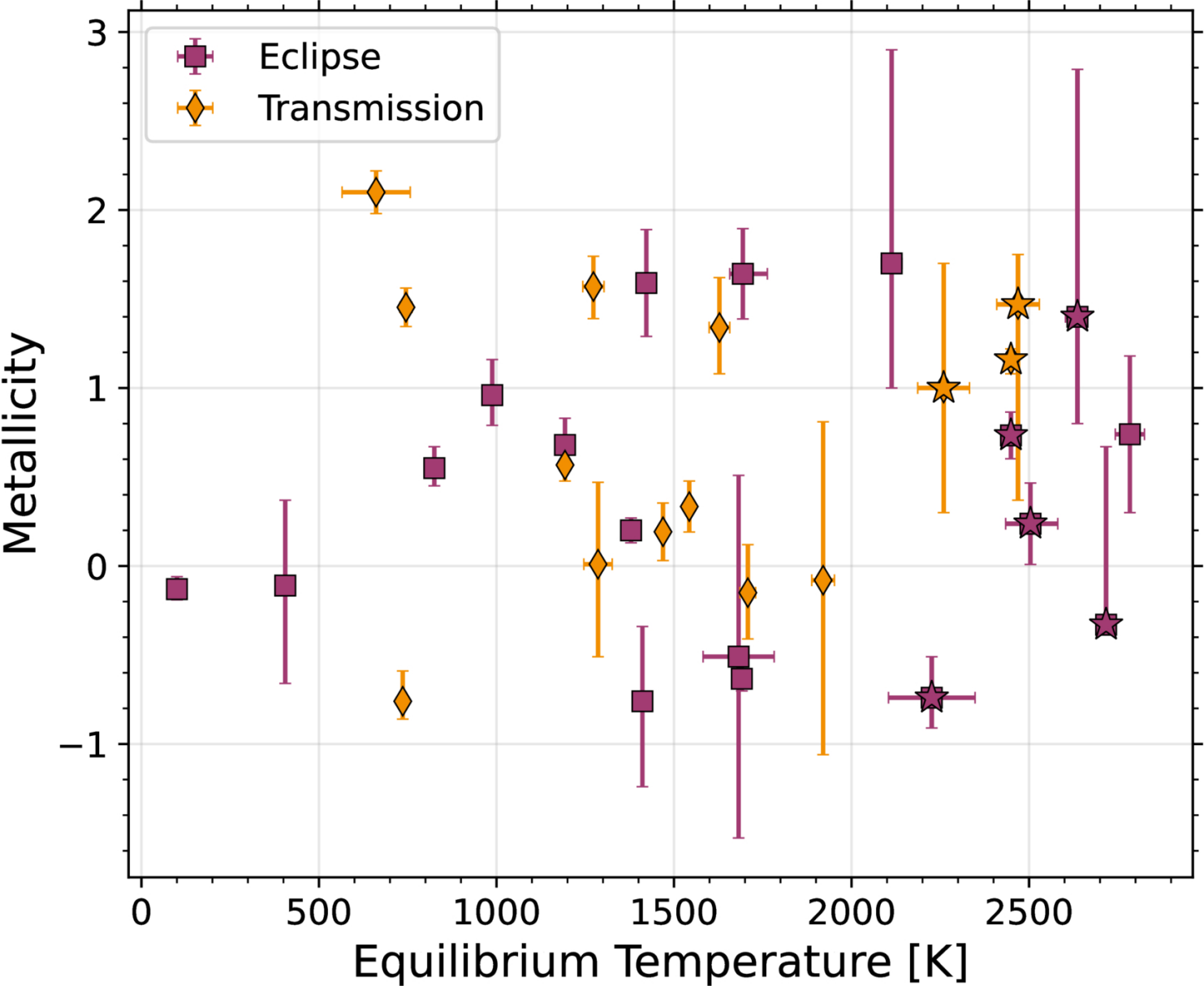
Figure 5. from Joshua D. Lothringer et al 2026 Astron. J. 171 doi:10.3847/1538-3881/ae1b8e https://dx.doi.org/10.3847/1538-3881/ae1b8e © 2025. The Author(s). Published by the American Astronomical Society.
