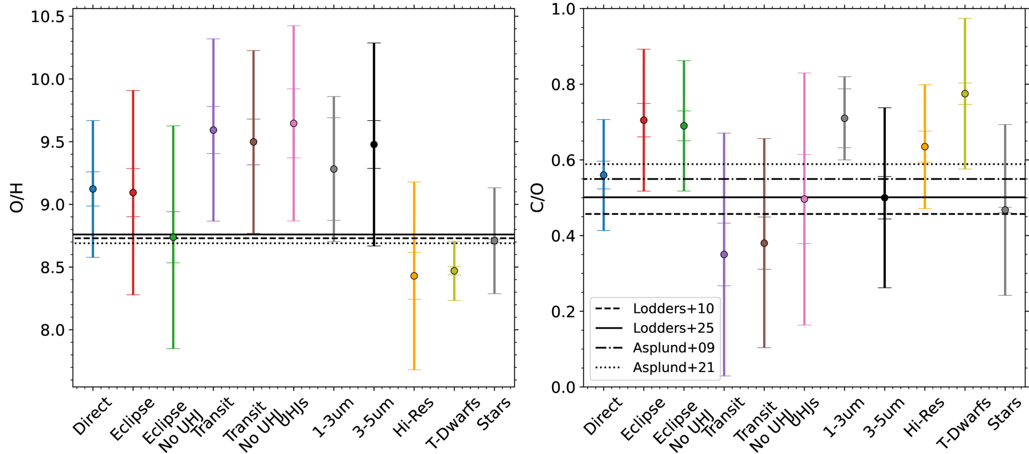
Figure 4. from Joshua D. Lothringer et al 2026 Astron. J. 171 doi:10.3847/1538-3881/ae1b8e https://dx.doi.org/10.3847/1538-3881/ae1b8e © 2025. The Author(s). Published by the American Astronomical Society.
