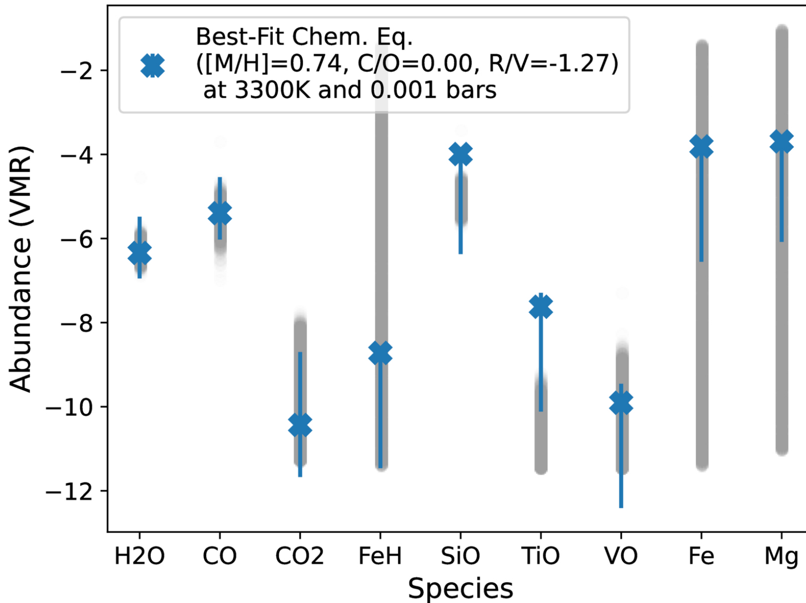
Figure 2. from Joshua D. Lothringer et al 2026 Astron. J. 171 doi:10.3847/1538-3881/ae1b8e https://dx.doi.org/10.3847/1538-3881/ae1b8e © 2025. The Author(s). Published by the American Astronomical Society.
