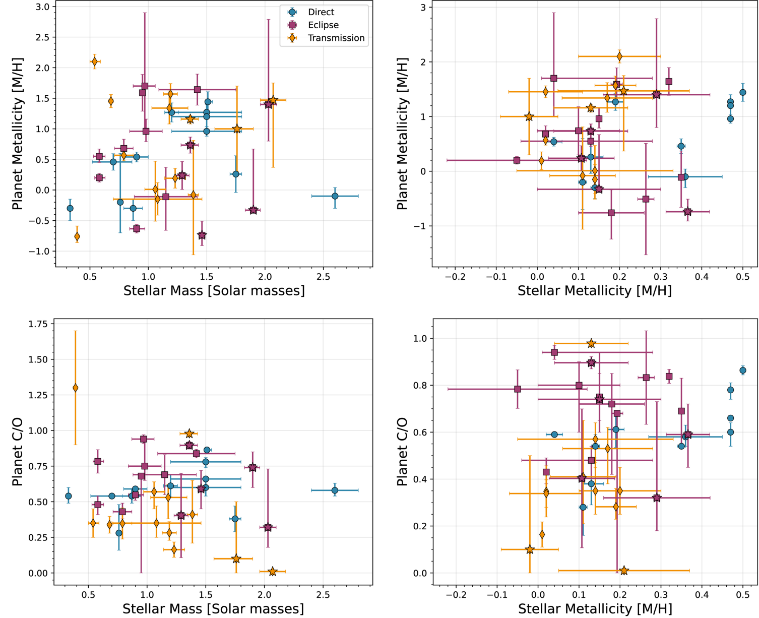
Figure 10. from Joshua D. Lothringer et al 2026 Astron. J. 171 doi:10.3847/1538-3881/ae1b8e https://dx.doi.org/10.3847/1538-3881/ae1b8e © 2025. The Author(s). Published by the American Astronomical Society.
