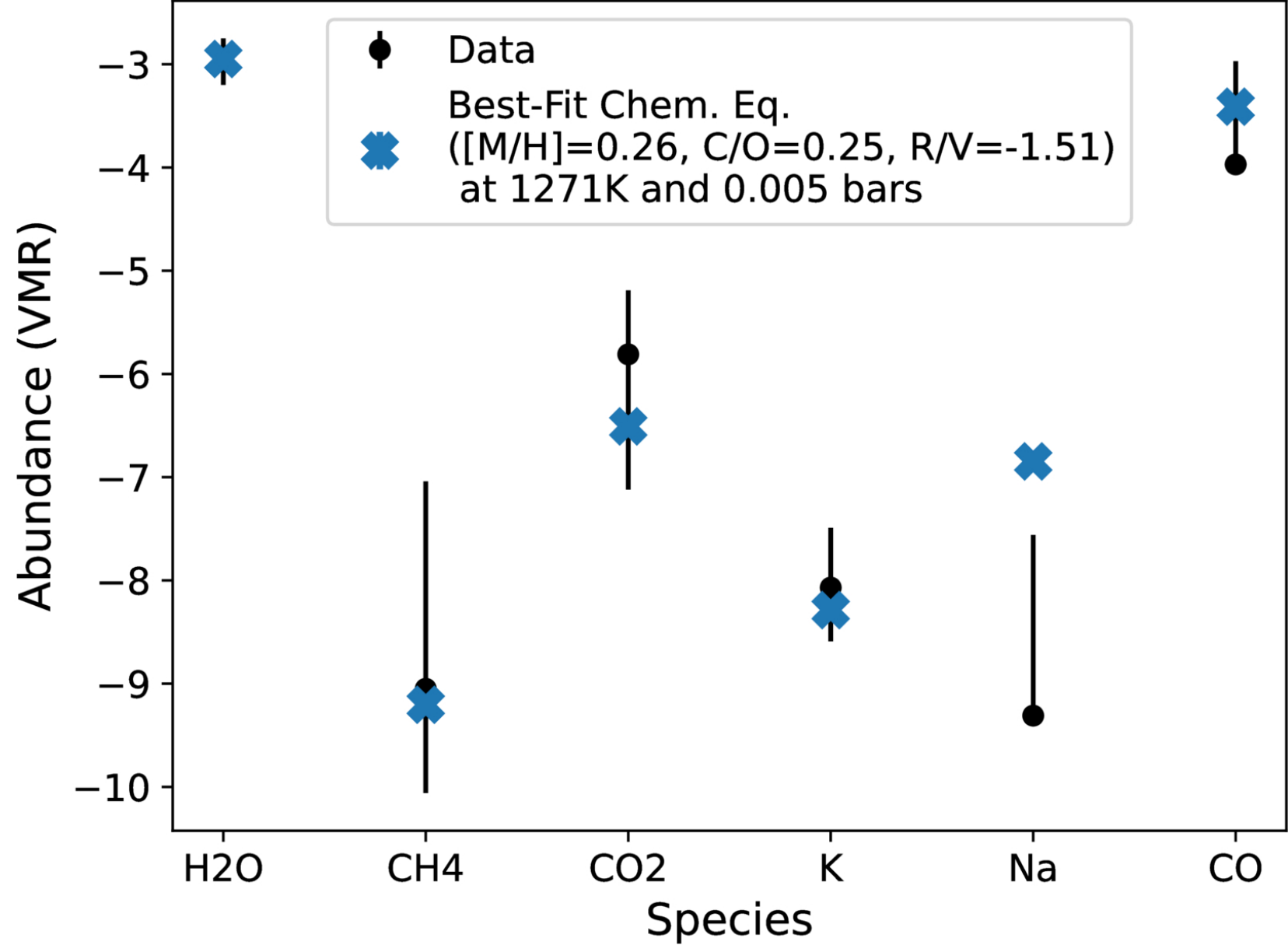
Figure 1. from Joshua D. Lothringer et al 2026 Astron. J. 171 doi:10.3847/1538-3881/ae1b8e https://dx.doi.org/10.3847/1538-3881/ae1b8e © 2025. The Author(s). Published by the American Astronomical Society.
