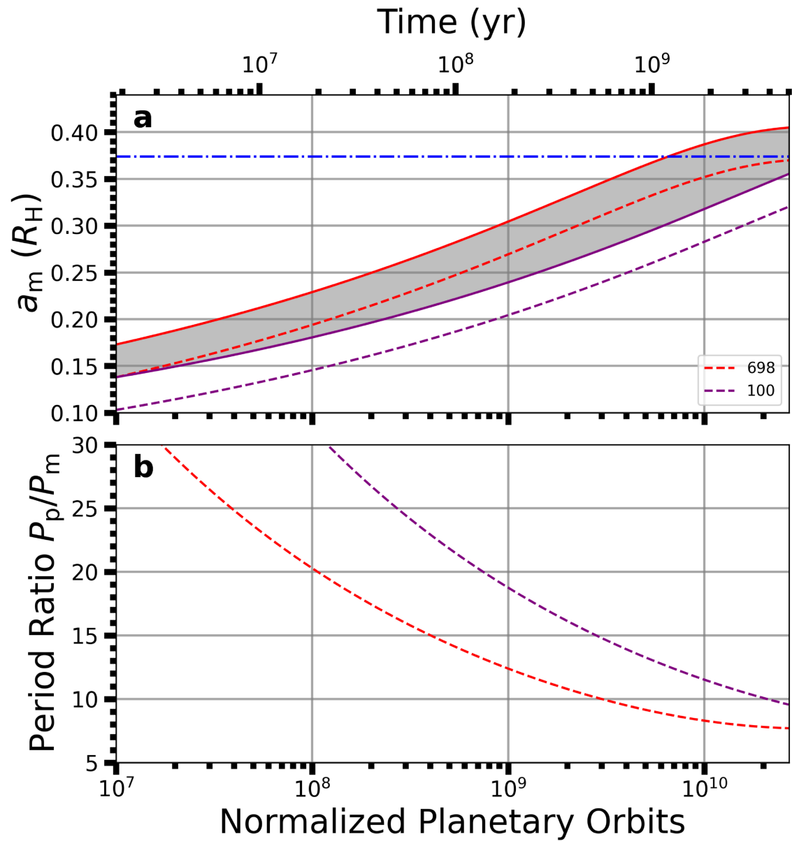
Figure 9. from Shaan D. Patel et al 2026 Astron. J. 171 doi:10.3847/1538-3881/ae1b8c https://dx.doi.org/10.3847/1538-3881/ae1b8c © 2025. The Author(s). Published by the American Astronomical Society.
