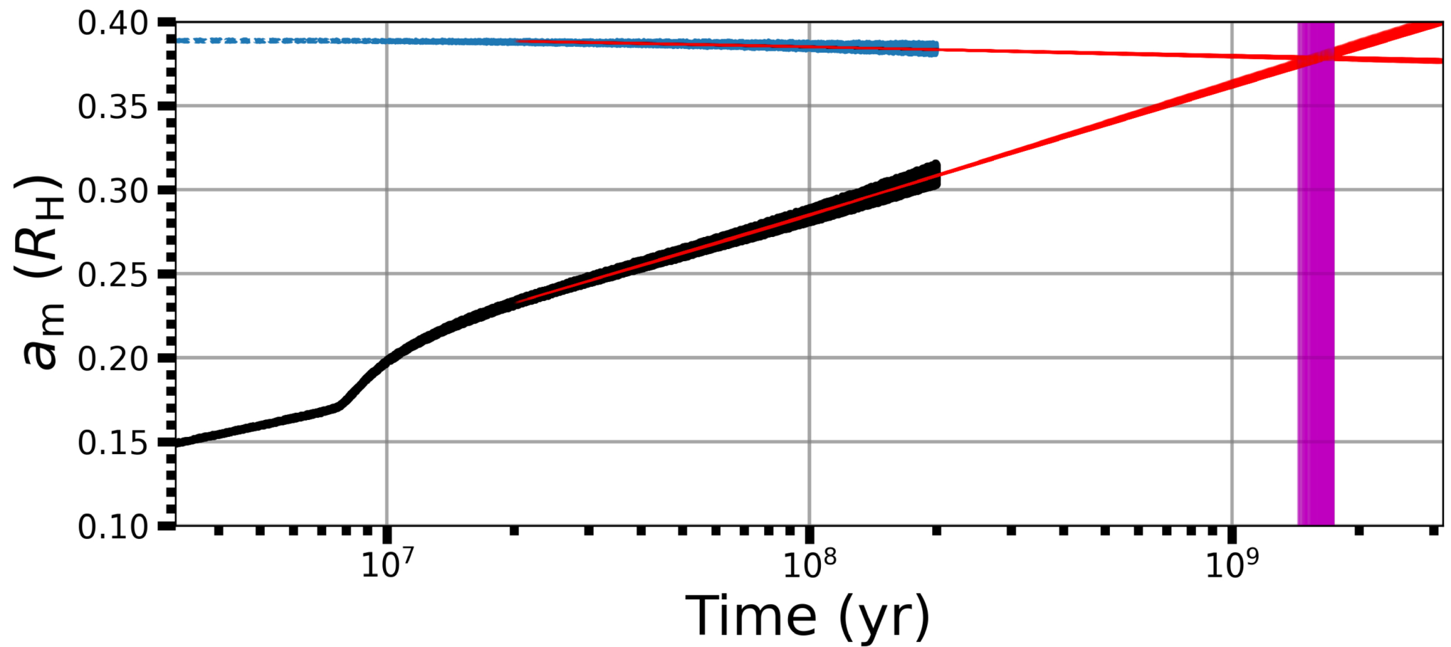
Figure 8. from Shaan D. Patel et al 2026 Astron. J. 171 doi:10.3847/1538-3881/ae1b8c https://dx.doi.org/10.3847/1538-3881/ae1b8c © 2025. The Author(s). Published by the American Astronomical Society.
