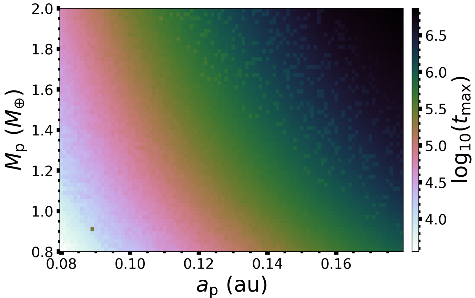
Figure 5. from Shaan D. Patel et al 2026 Astron. J. 171 doi:10.3847/1538-3881/ae1b8c https://dx.doi.org/10.3847/1538-3881/ae1b8c © 2025. The Author(s). Published by the American Astronomical Society.
