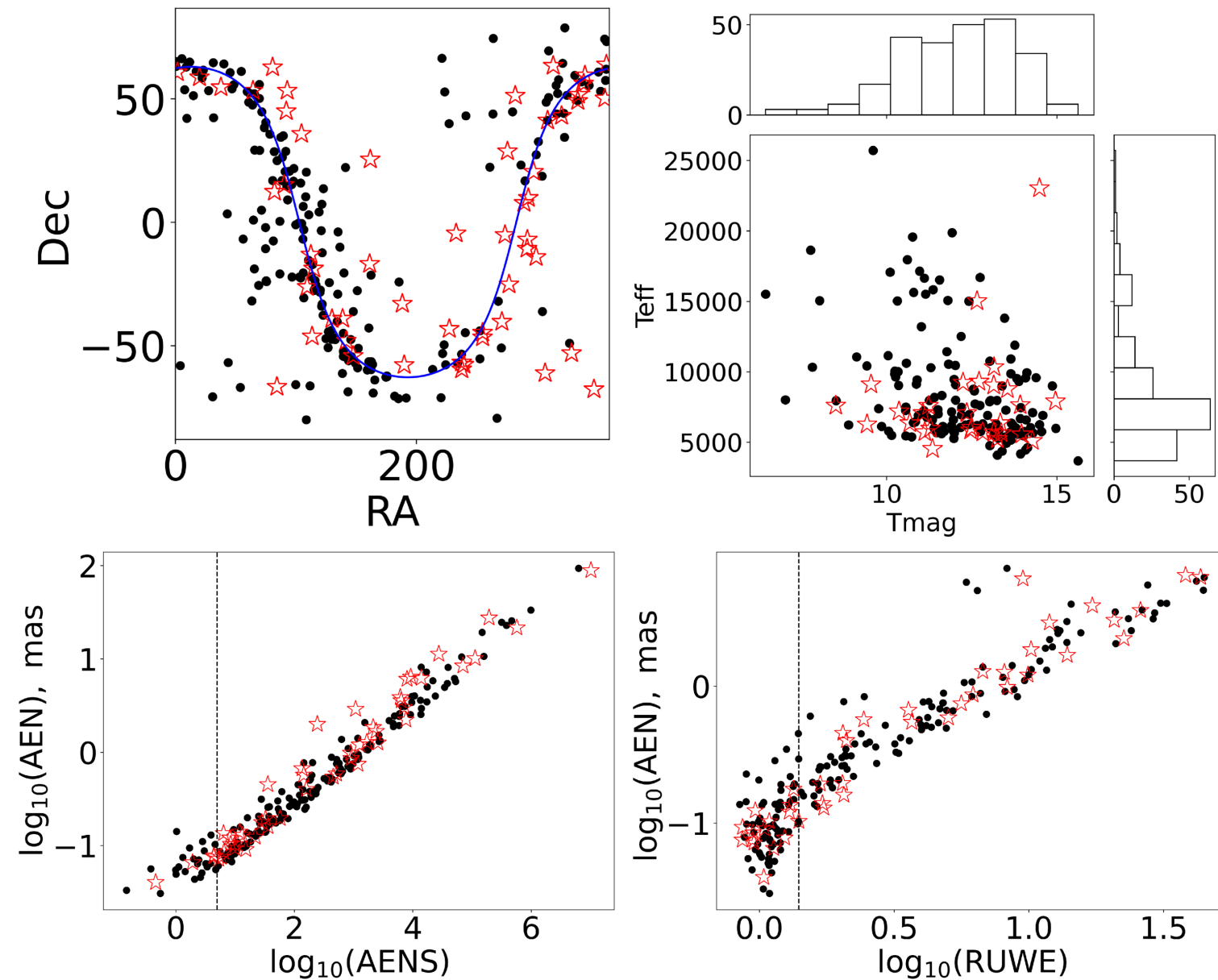
Figure 9. from V. B. Kostov et al 2026 Astron. J. 171 doi:10.3847/1538-3881/ae1b8a https://dx.doi.org/10.3847/1538-3881/ae1b8a © 2025. The Author(s). Published by the American Astronomical Society.
