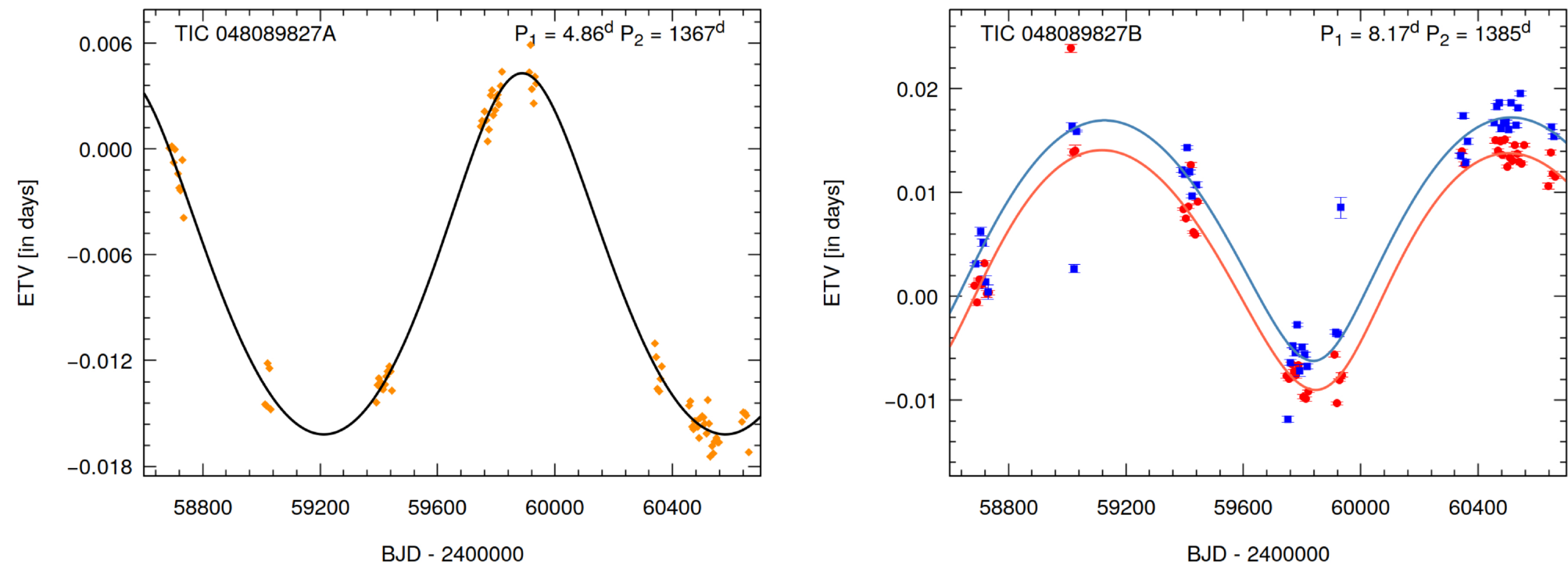
Figure 8. from V. B. Kostov et al 2026 Astron. J. 171 doi:10.3847/1538-3881/ae1b8a https://dx.doi.org/10.3847/1538-3881/ae1b8a © 2025. The Author(s). Published by the American Astronomical Society.
