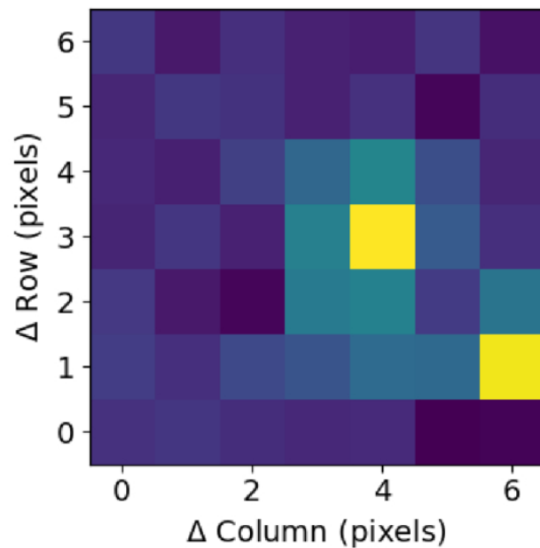
Figure 4. from V. B. Kostov et al 2026 Astron. J. 171 doi:10.3847/1538-3881/ae1b8a https://dx.doi.org/10.3847/1538-3881/ae1b8a © 2025. The Author(s). Published by the American Astronomical Society.
