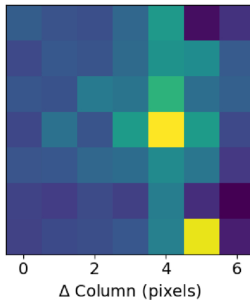
Figure 4. from V. B. Kostov et al 2026 Astron. J. 171 doi:10.3847/1538-3881/ae1b8a https://dx.doi.org/10.3847/1538-3881/ae1b8a © 2025. The Author(s). Published by the American Astronomical Society.
