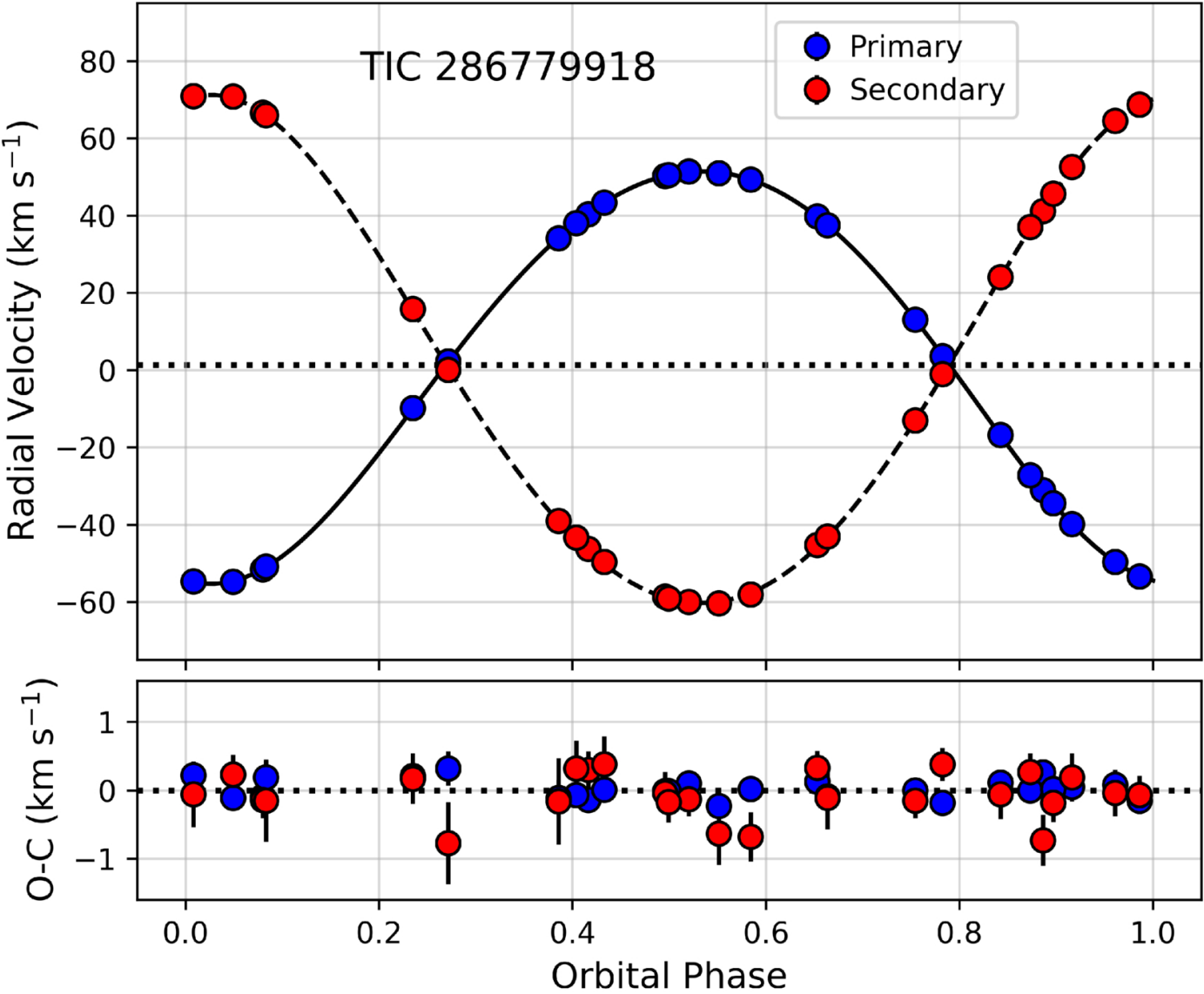
Figure A5. from V. B. Kostov et al 2026 Astron. J. 171 doi:10.3847/1538-3881/ae1b8a https://dx.doi.org/10.3847/1538-3881/ae1b8a © 2025. The Author(s). Published by the American Astronomical Society.
