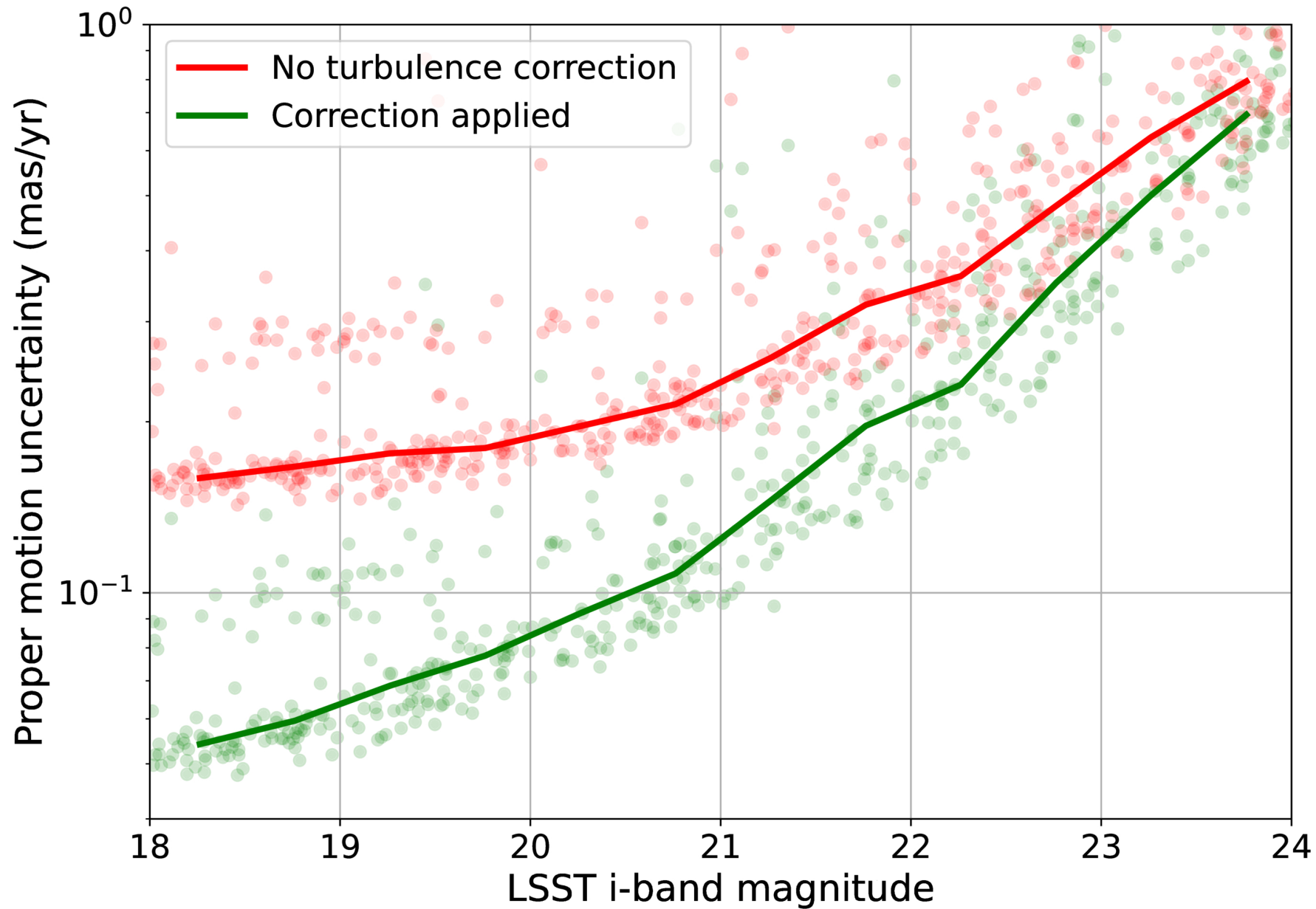
Figure 6. from Daniel C. H. Gomes et al 2025 Astron. J. 170 doi:10.3847/1538-3881/ae1a7b https://dx.doi.org/10.3847/1538-3881/ae1a7b © 2025. The Author(s). Published by the American Astronomical Society.
