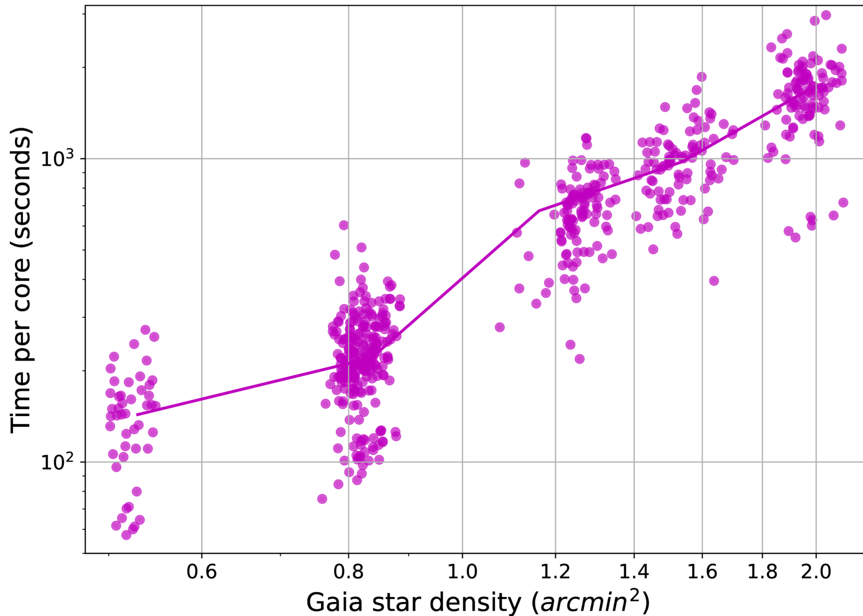
Figure 4. from Daniel C. H. Gomes et al 2025 Astron. J. 170 doi:10.3847/1538-3881/ae1a7b https://dx.doi.org/10.3847/1538-3881/ae1a7b © 2025. The Author(s). Published by the American Astronomical Society.
