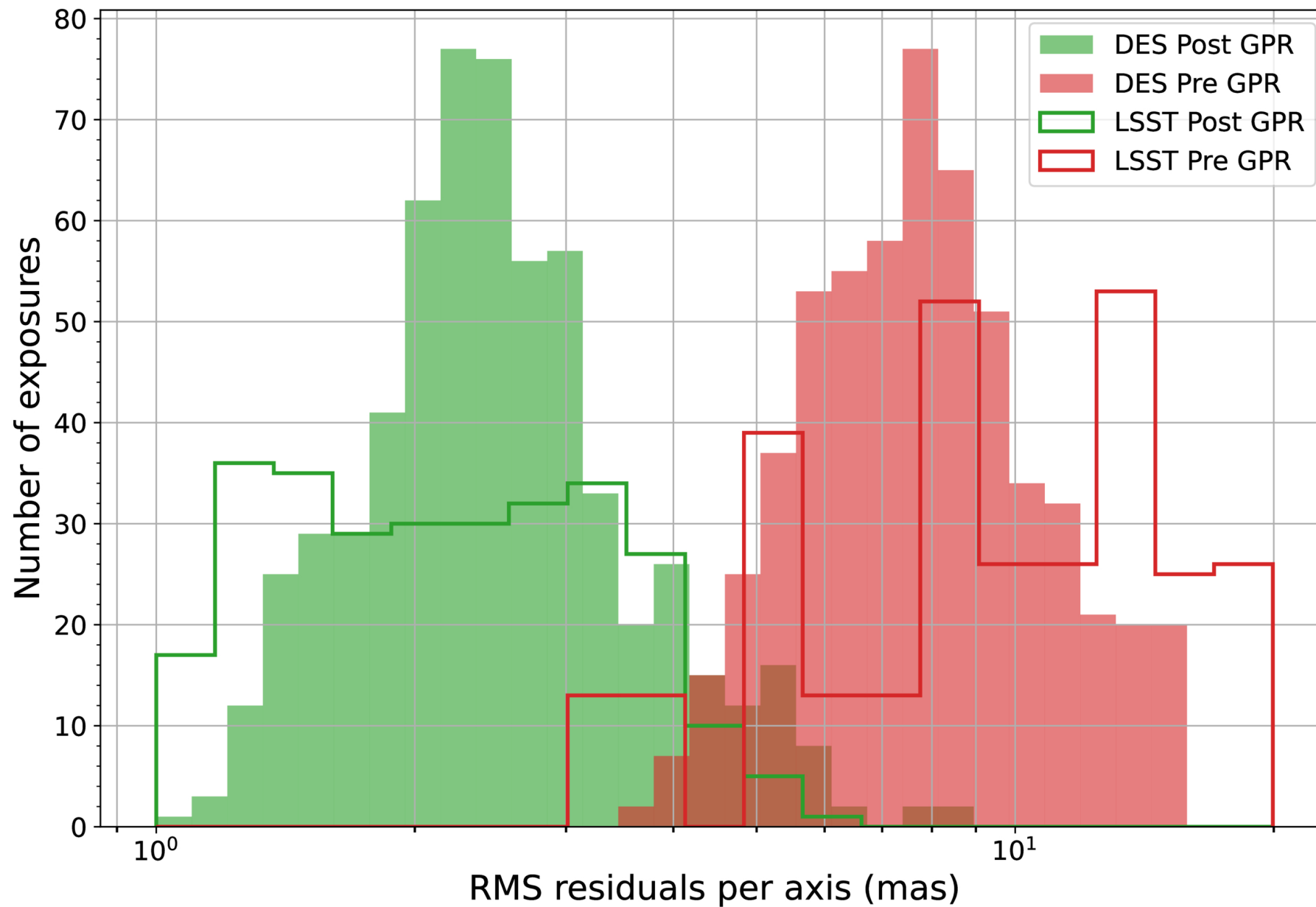
Figure 2. from Daniel C. H. Gomes et al 2025 Astron. J. 170 doi:10.3847/1538-3881/ae1a7b https://dx.doi.org/10.3847/1538-3881/ae1a7b © 2025. The Author(s). Published by the American Astronomical Society.
